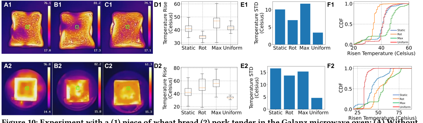
Figure 10: Experiment with a (1) piece of wheat bread (2) pork tender in the Galanz microwave oven: (A) Without metasurface; (B) Metasurface maximizes energy; (C) Metasurface uniformes heat; (D) Box plot of temperature shows with uniform heating, the standard deviation of temperature greatly decreases without metasurface; (E) When maximizing energy, the temperature is 2°C/7.4°C/8°C higher; (F) CDF of temperature.
